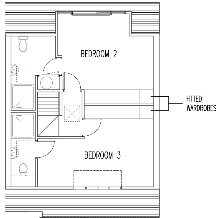
SECOND FLOOR
